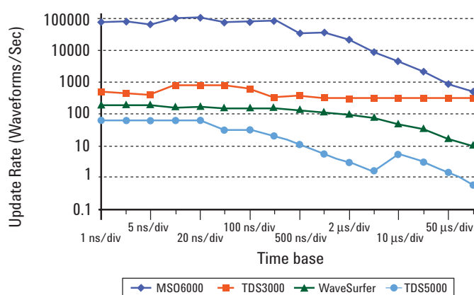
Figure 6. Waveform update rates in comparison using each scope's default real-time acquisition mode.
