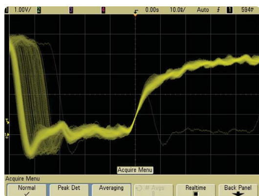
Figure 5. 256 levels of display intensity gradation shows characteristics of jitter, noise, and signal anomalies on Agilent's 6000 Series oscilloscope.
